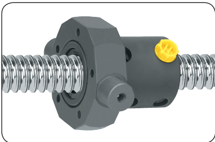
SX nut with trunnions flange (FHTF)
