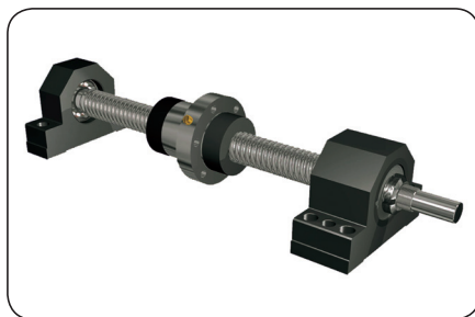
Complete ball screw assembly with support bearing
