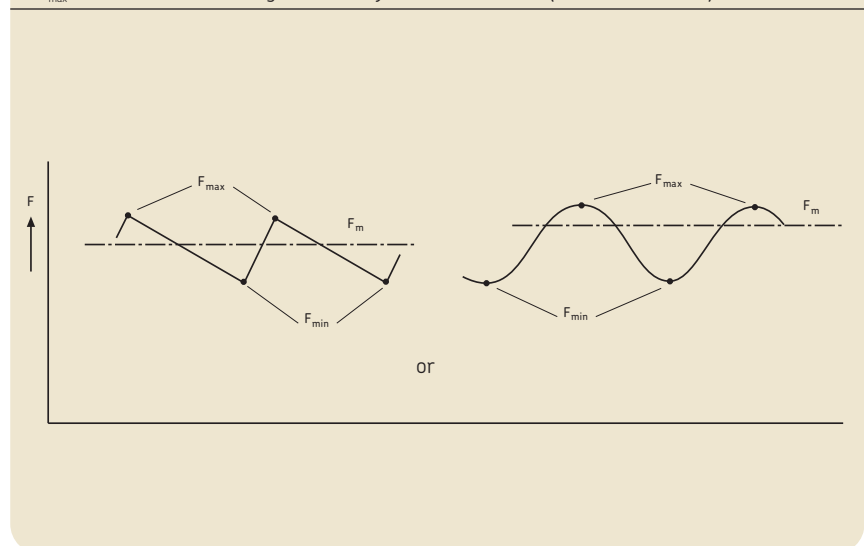
Fig 2.3: Mean load F_m at constant maximum and minimum forces (approximation) F_{max} to be used when taking static safety into consideration (see also table 2.8)
