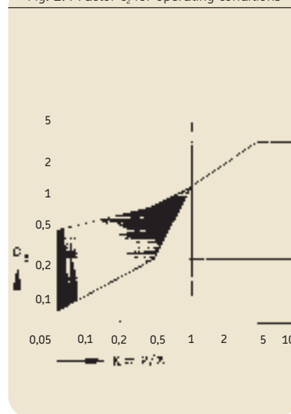
Fig. 2.4 Factor c_2 for operating conditions
