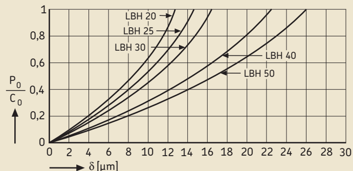
Fig. 3.10 Elastic deformation of clearance-free linear ball bearings in the ball contact zone
