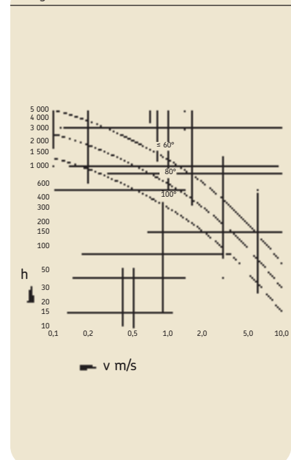
Fig. 2.7 Relubrication intervals
