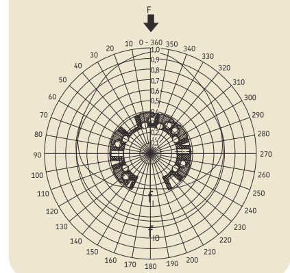
Fig. 3.5 Factor f_i and f_{i0} influence of the direction of load for LBCT and LBCF linear ball bearings
