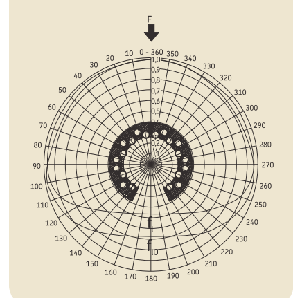
Fig. 3.6 Factors f_i and f_{i0} influence of the direction of load for LBHT linear ball bearings
