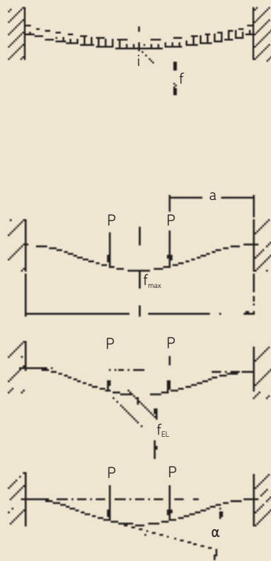
Fig. 3.7 Deflection and misalignment of freely supported and clamped steel shafts. Calculated using E = 206\,000\text{ N/mm}^2 and r = 77\,000\text{ N/m}^3
