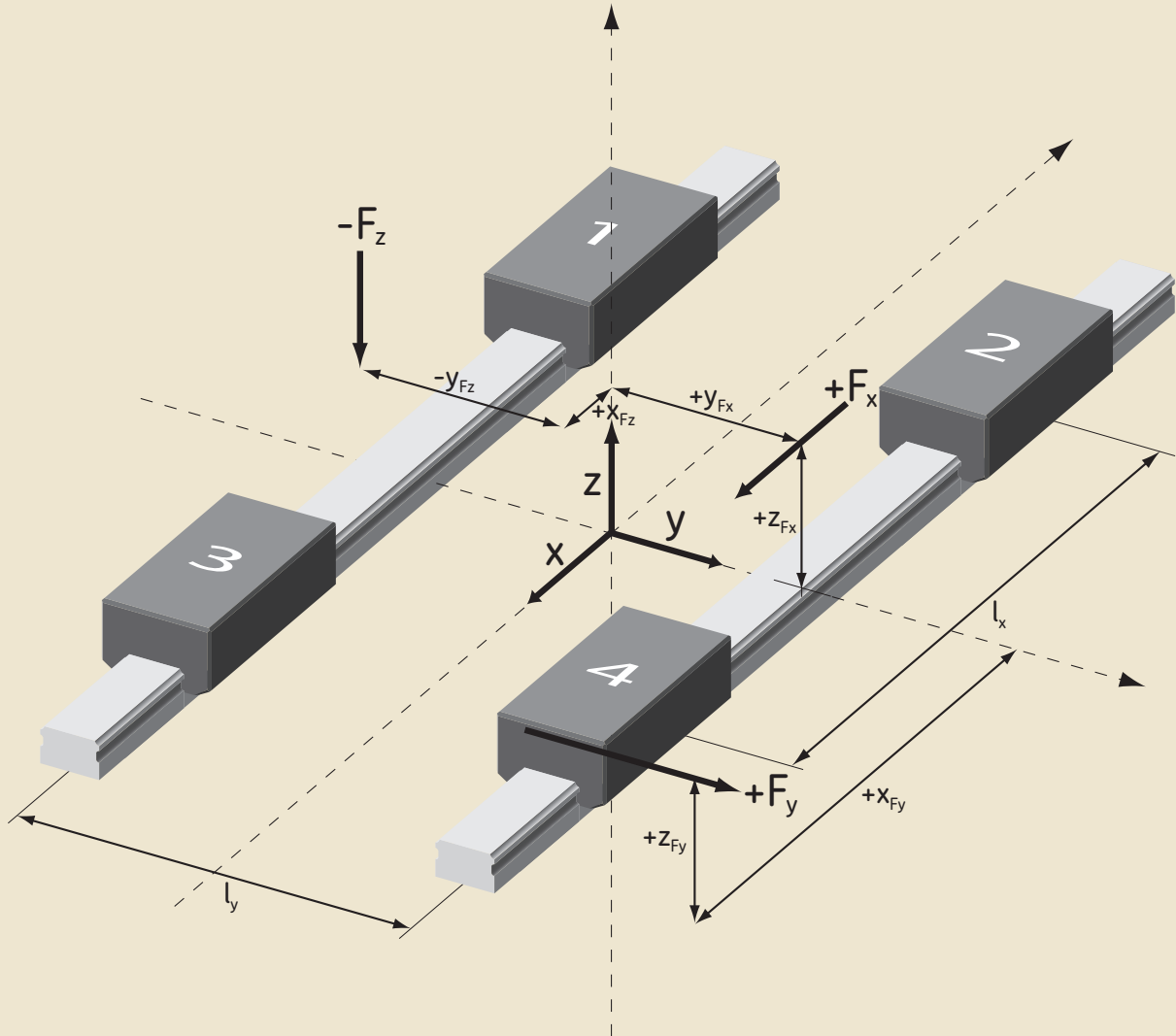
Fig. 2.1 Schematic representation of a carriage incl. definition of directions
