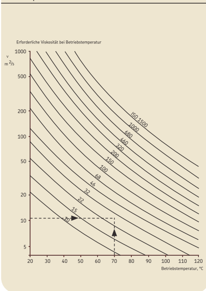
Fig. 2.6 Lubricant viscosity v vs. temperature t
