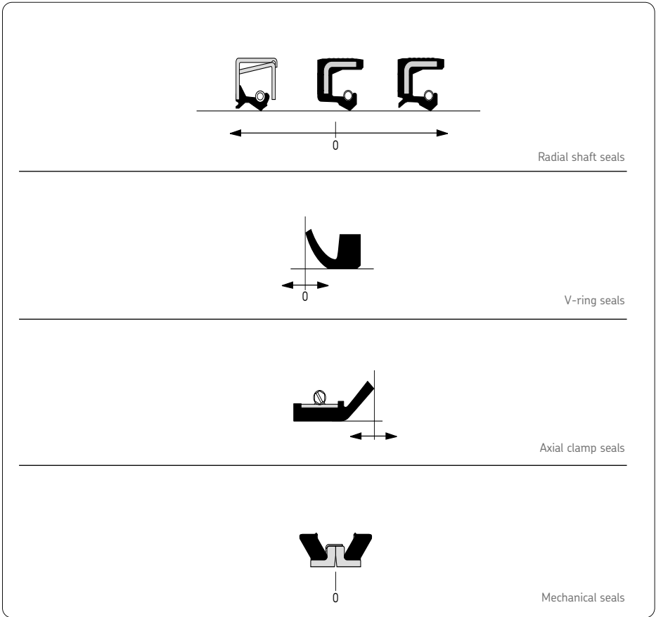
Fig 34. Axial movement
